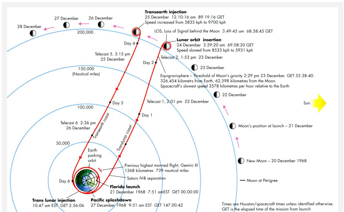
Plan of the trajectory to the Moon followed by Apollo 8.
