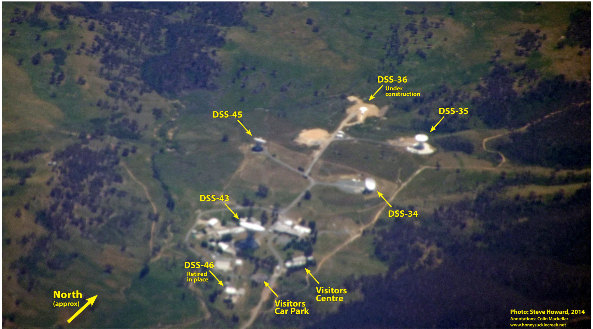
The Canberra Deep Space Communication Complex as viewed from a commercial airliner flying between Sydney and Melbourne at approximately 10,000 metres. (The image is foreshortened.)
